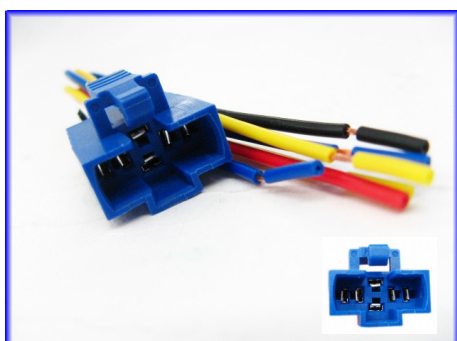
22mm 6P 1no 1nc YIJIA-M22-6P 14200414
