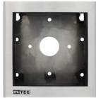
MEM-FS10 1 Unit Flush Mount 128W x 132H x 40D mm
