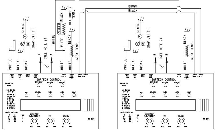
MIX REF. SYSTEM (DANFOSS TL36 COMPRESSOR)
