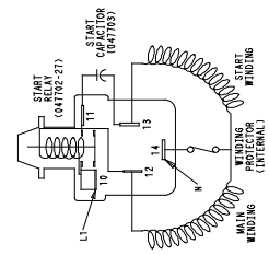
COMPRESSOR WIRING (MODEL TL3G W/HST) FIG. 3
