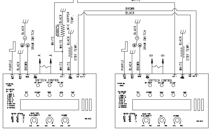
MIX REF. SYSTEM (DANFOSS TL3A COMPRESSOR) FIG. 1
