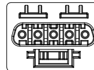
Connector pin view 2:1
