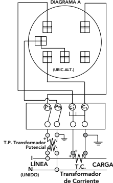
DIAGRAM A 1Ø2W with 1 P.T.'s & 1 C.T. Single Stator Meter(2W1Ø) - Form 3S 5T Socket, Test Switch #TS04-0101
