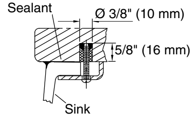
Solid-Surface Installation
