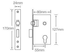
QS6055/3 Adjustable rollerbolt + deadbolt 55mm backset 60mm centre
