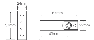
QS6002 Spring bolt
