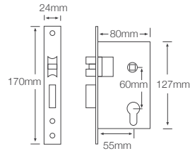
QS6055/1 Latch + deadbolt 55mm backset 60mm centre
