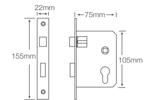
QS5757/5 Bathroom lock for 8mm spindle 57mm backset 57mm centre
