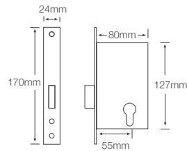
QS6055/4 Deadbolt 55mm backset
