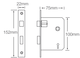
QS5757/2 two lever 57mm backset 57mm centre
