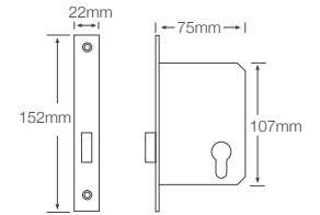
QS6057/4 Cylinder deadbolt 57mm backset
