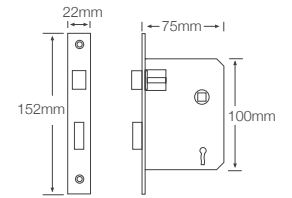
QS5757 Stainless steel forend – three lever 57mm backset 57mm centre
