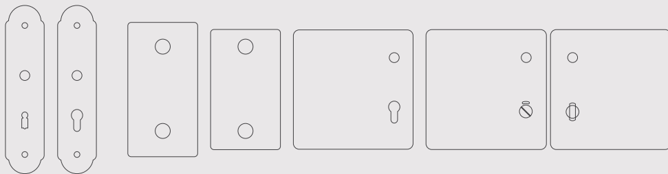
QS4489 QS4487 QS4486 QS4485 QS4485 KH 200x48x57mm 190x100mm 170x100mm 170x170mm with WC indicator CYL 200x48x60mm supplied with supplied with QS2205/1 QS2203/1
