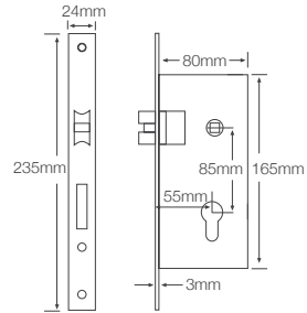
QS8555 Timber latch and double throw deadbolt 55mm backset 85mm centre
