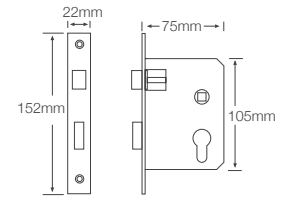
QS5757/1 Cylinder latch lock + deadbolt 57mm backset 60mm centre
