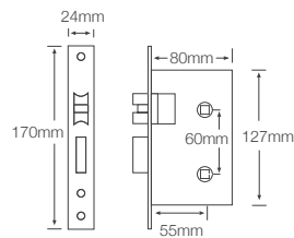
QS6055/5 Bathroom lock 55mm backset 60mm centre
