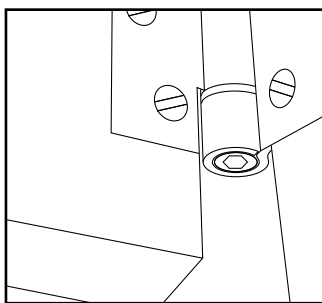
Loosen grub screw A Attach hinge to door
