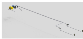
Suspension_Pneumatic_System
