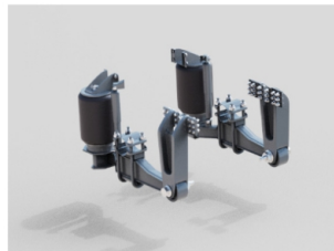
Rear_Suspension_Support_Pneumatic
