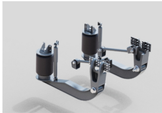
Front_Suspension_Support_Front
