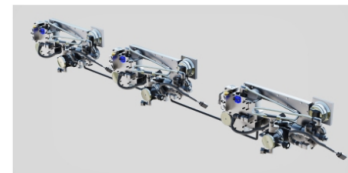
H2-Tank_Components
