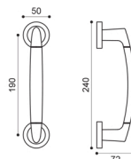
AT 20 Maniglione. Pull handle.
