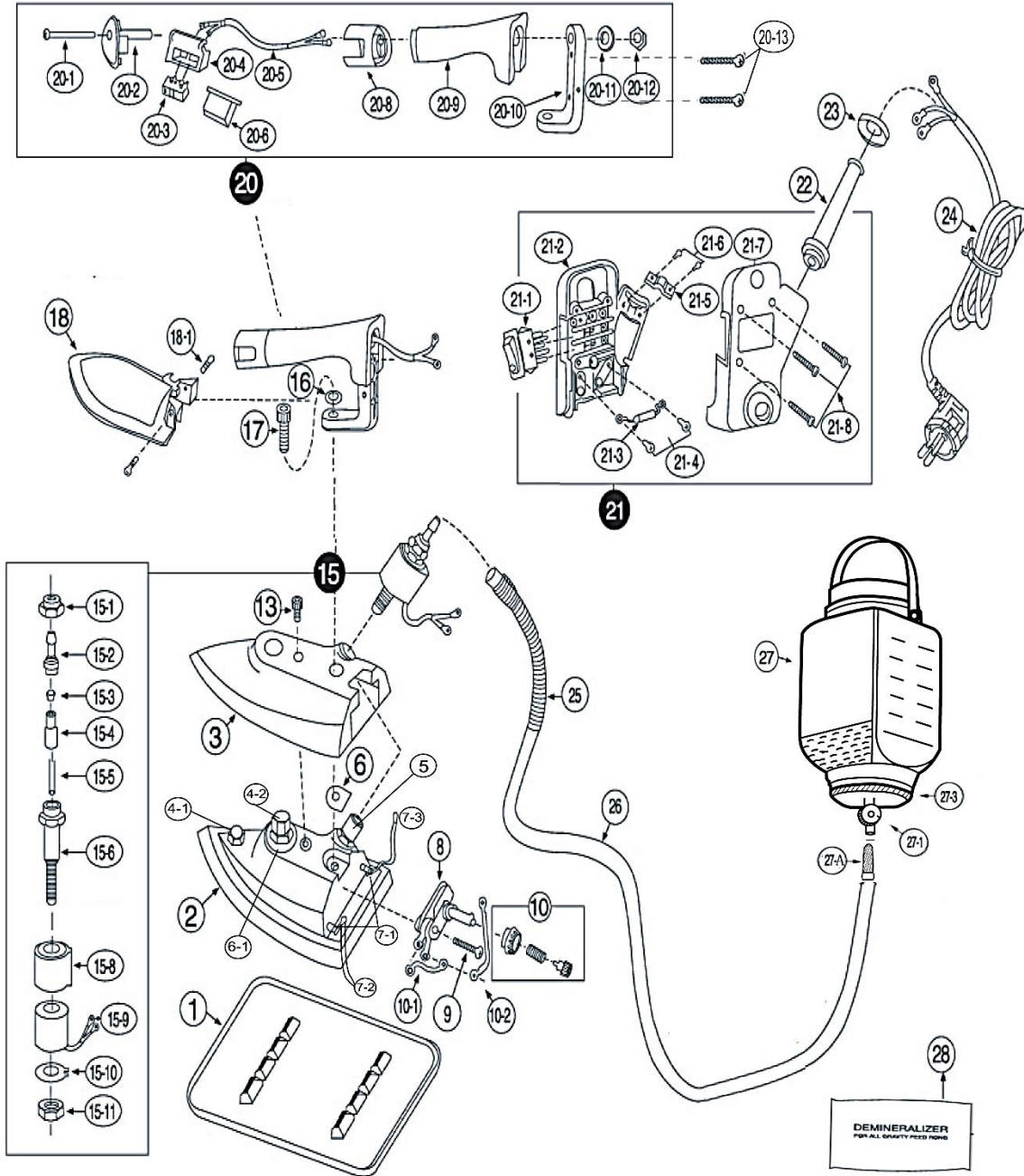
Exploded View Model SGB700
