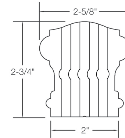
6710B Profile
