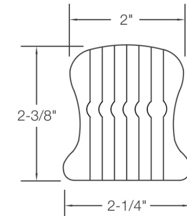
9200B Profile
