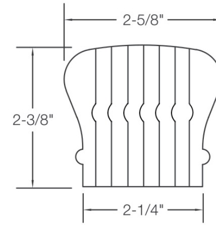
6210B Profile
