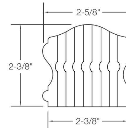
8500B Profile
