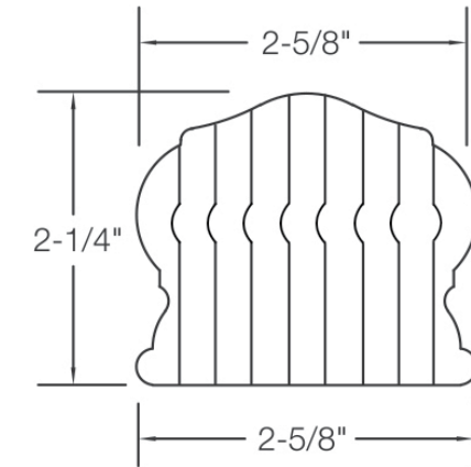
8200B Profile
