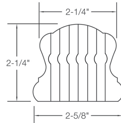
8000B Profile
