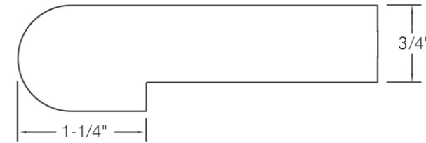
8093 Profile
