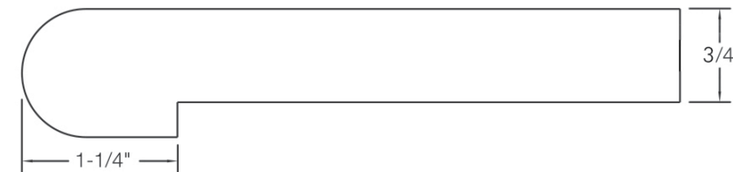
8095 Profile
