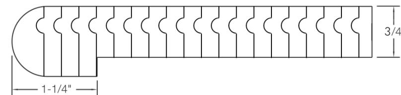
Bending Nosing
