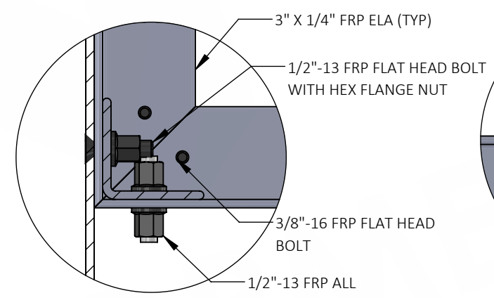
DETAIL E SCALE 1 : 4
