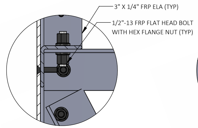
DETAIL C SCALE 1 : 4
