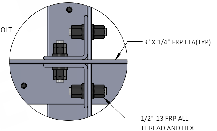
DETAIL F SCALE 1 : 4
