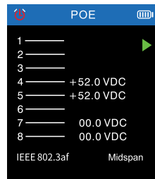
Midspan
