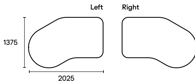
30 degree corner
