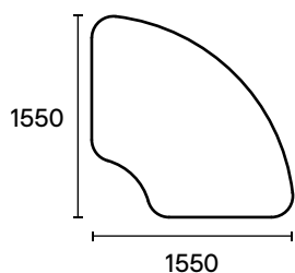
90 degree curve
