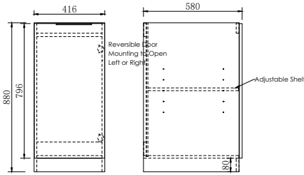
Byron Black Oak Floor Cabinet 416mm 1 Door With Handle
