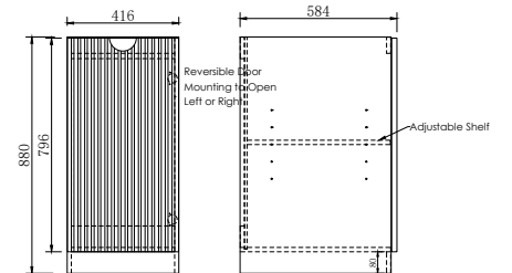
Marlo Floor Cabinet 416mm 1 Door With Handle
