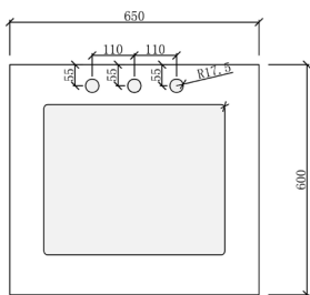
Back View Pre Semi-Drilling Tapholes
