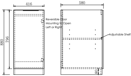
Byron Natural Oak Floor Cabinet 416mm 1 Door With Handle
