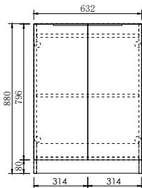
Byron Natural Oak Floor Cabinet 632mm 2 Doors With Handles
