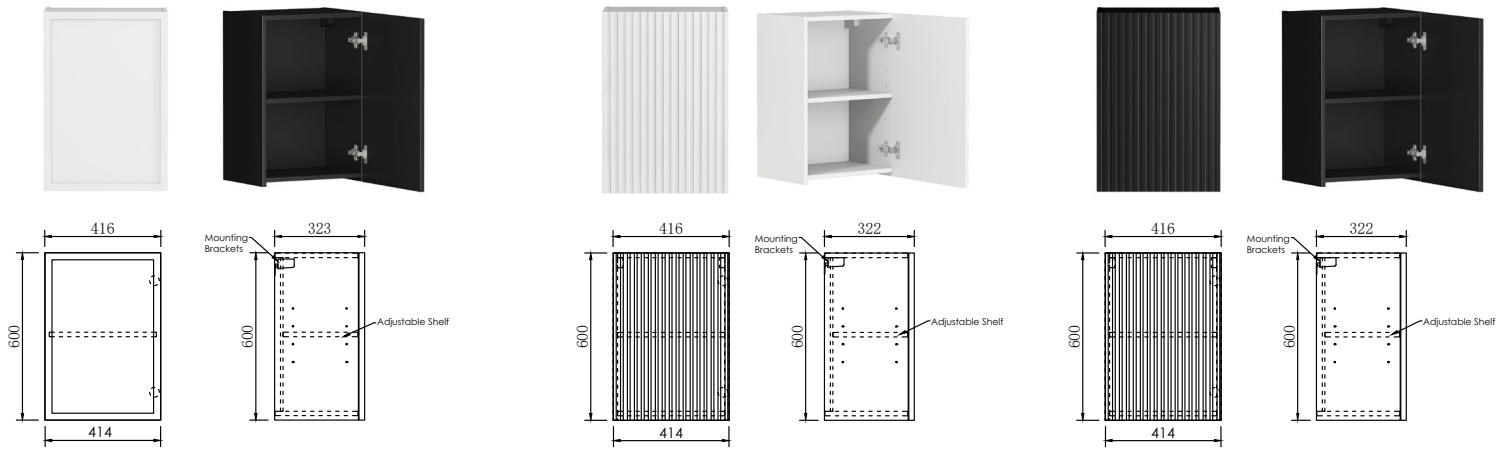
Hampshire Matte White & Matte Black Wall Cabinet 416mm Singer Door Bevel Finger Pull
