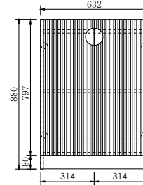
Marlo Floor Cabinet 632mm 2 Doors With Handles
