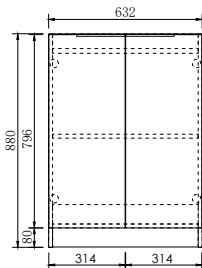
Byron Black Oak Floor Cabinet 632mm 2 Doors With Handles
