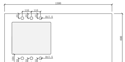
Back View Pre Semi-Drilling Tapholes
