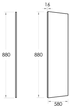
A Floor Cabinets End Panel 880x580x16mm
