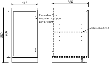
Hampshire Matte White & Matte Black Floor Cabinet 416mm 1 Door Bevel Finger Pull
