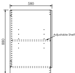
Byron Natural Oak Floor Cabinet 632mm 2 Doors With Handles
