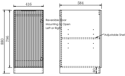
Noosa Matte White Floor Cabinet 416mm 1 Door With Handle
