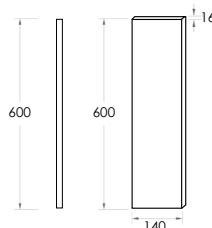
Wall Cabinets Filler 600x140x16mm
