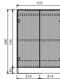
Bondi Floor Cabinet 632mm 2 Doors With Handles
