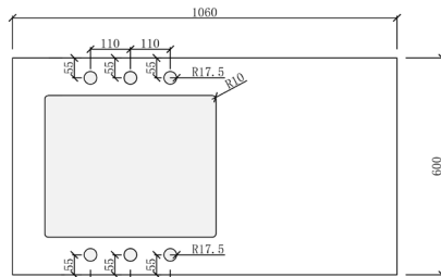
Back View Pre Semi-Drilling Tapholes
