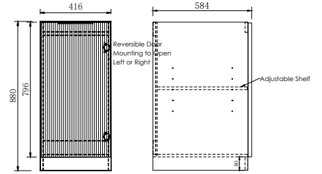
Bondi Floor Cabinet 416mm 1 Door With Handle
