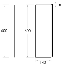
B Wall Cabinets Filler Panel 600x140x16mm Cut to Size on Site
