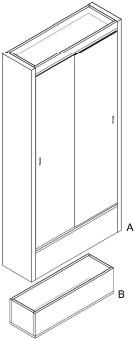
A : Quartz Retail Unit B : Floor fixing block
