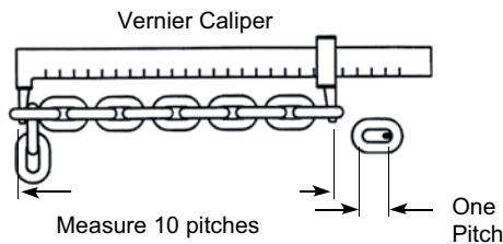
Figure 8: Chain Inspection
