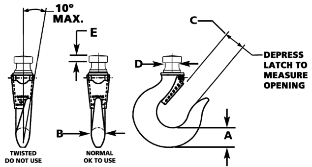
Figure 3 – Hook Inspection
