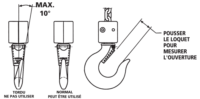
Figure 3 – Inspection du crochet
