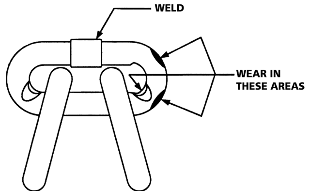
Figure 4 - Chain Inspection
