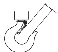
Figure 5 - Inspection du crochet
