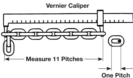
Figure 7 - Chain Inspection
