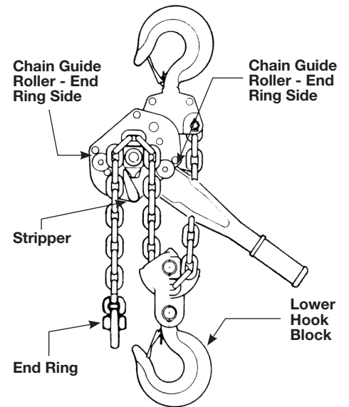
Figure 11 - Reeving - 6 Ton
