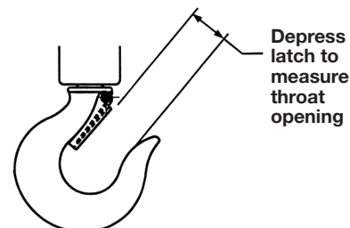
Figure 5 - Hook Inspection
