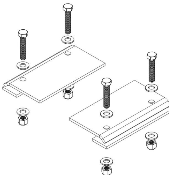
I-Beam Clamps & I-Beam Bolt Kit (2) I-Beam Clamps (2) I-Beam Shims (4) Hex Bolts 1/2"-13x2-1/2" (8) Washers, 1/2" Flat (4) Hex Nuts 1/2"-13, Nylon Lock
