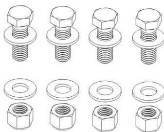
Universal Mount Bolt Kit (4) Hex Bolts 1/2"-13x1-1/2" (8) Washers, 1/2" Flat (4) Hex Nuts 1/2"-13, Nylon Lock
