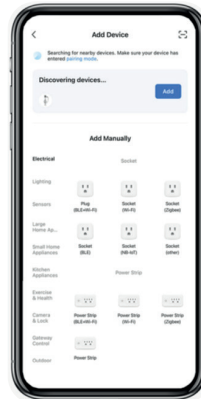
2-Search Device
