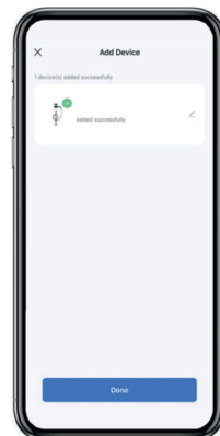
4-Added Successfully
