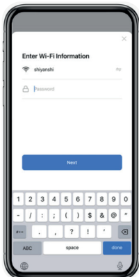
3-Enter Password
