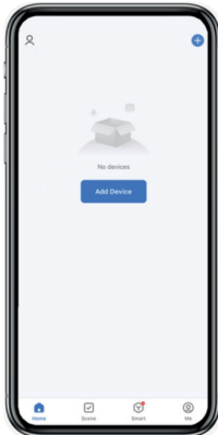
1-Add Device
