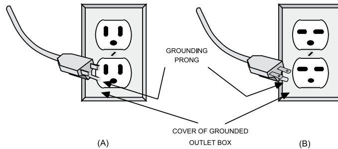
FIGURE 1: GROUNDING METHODS
