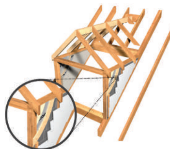
Timber frame wall with weatherboards
