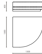
DW532 sx left DW533 dx right 1300 x 1300 x 400 mm 51,18 x 51,18 x 15,75 in
