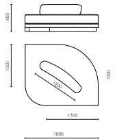
DW538 sx left DW539 dx right 1800 x 1500 x 650 mm 70,87 x 59,06 x 25,59 in
