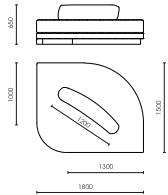
DW534 sx left DW535 dx right 1800 x 1500 x 650 mm 70,87 x 59,06 x 25,59 in
