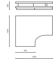
DW543 sx left DW544 dx right 1800 x 1500 x 380 mm 70,87 x 59,06 x 14,96 in
