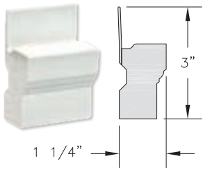
WM 180 Brickmould with Flange
