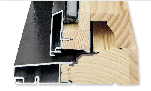
Casement Operating
