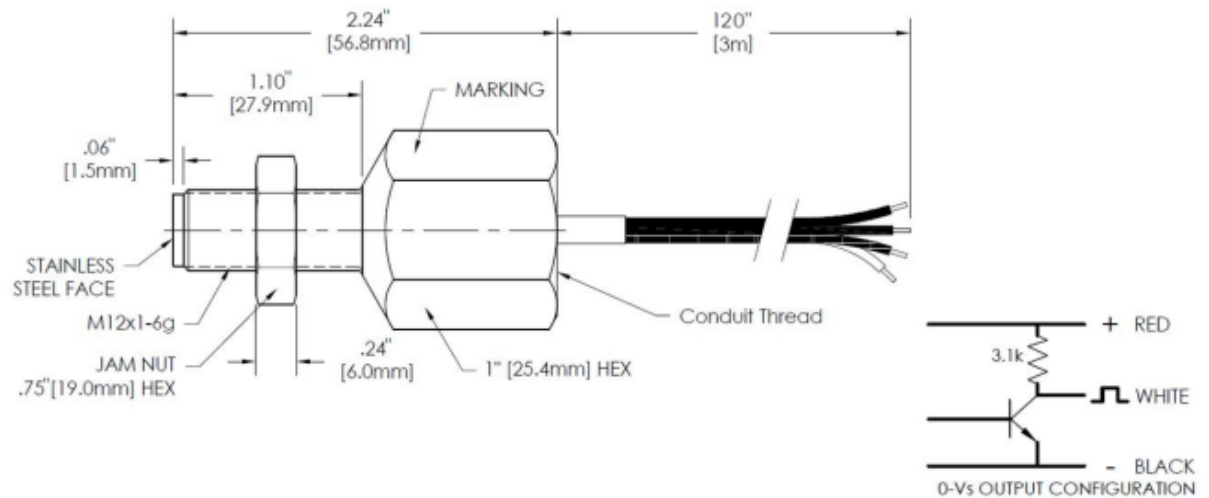
Figure 2. Sensor and Cable Assembly
