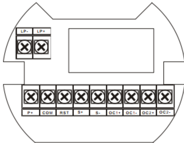
Figure 1. Connector Board
