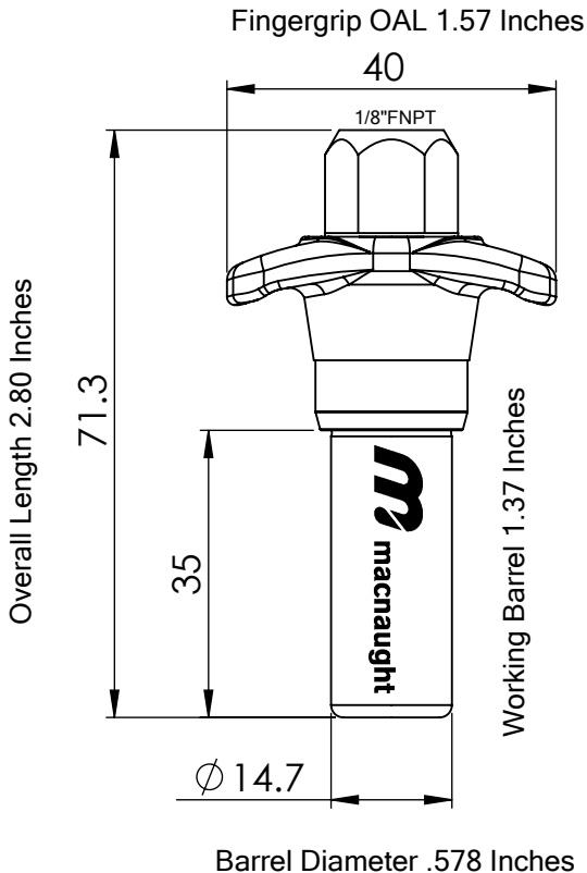
Macnaught USA KYPLUS-02 Dimensional
