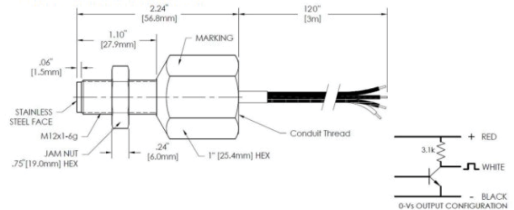
Figure 2. Sensor and Cable Assembly
