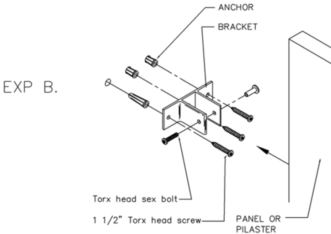
PANEL AND/OR PILASTER TO WALL ATTACHMENT STIRRUP BRACKET SHOWN
