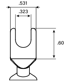
U-Spade Dimensions (in.)
