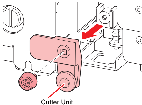
Cutter Unit
