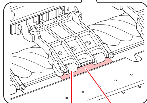
Pinch roller
