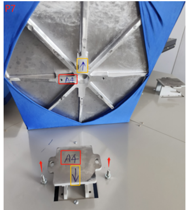
P7: Install the platen, match the mark (A4-A4) and the direction. We pre-aligned the platen to make it parallel to the heat plate to ensure the best pressure distribution. Fix the platen with screw, spring washer and flat washer.
