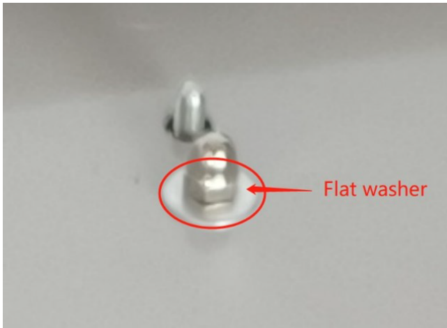
P5: Fix the four covers with screws as shown in the picture.
