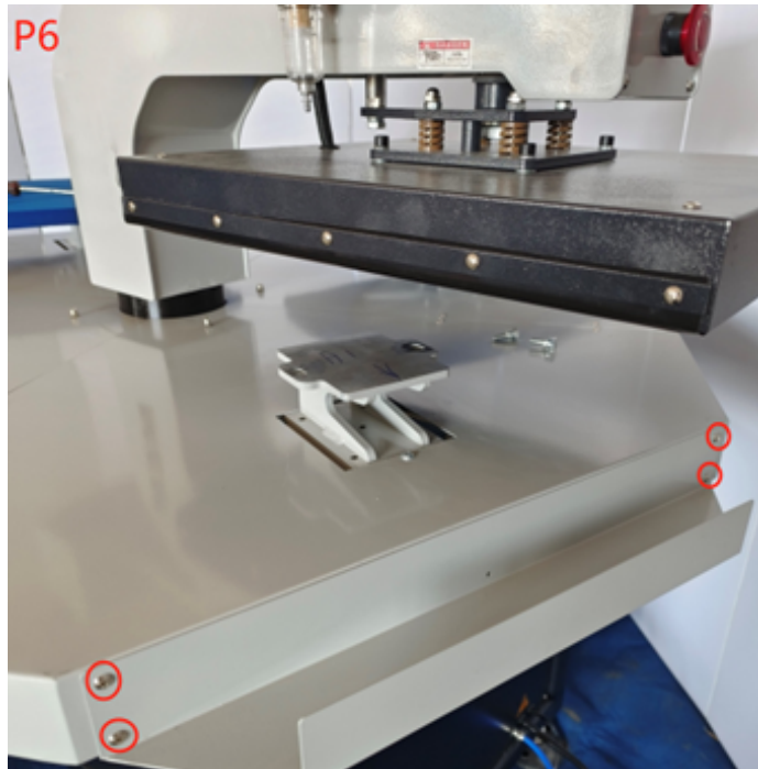
P6: Install the fabric tray (it is designed for long fabric press job, which can prevent the fabric from fall off, this part might not needed for regular t-shirt press)
