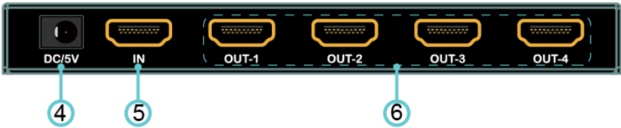
Rear Panel
