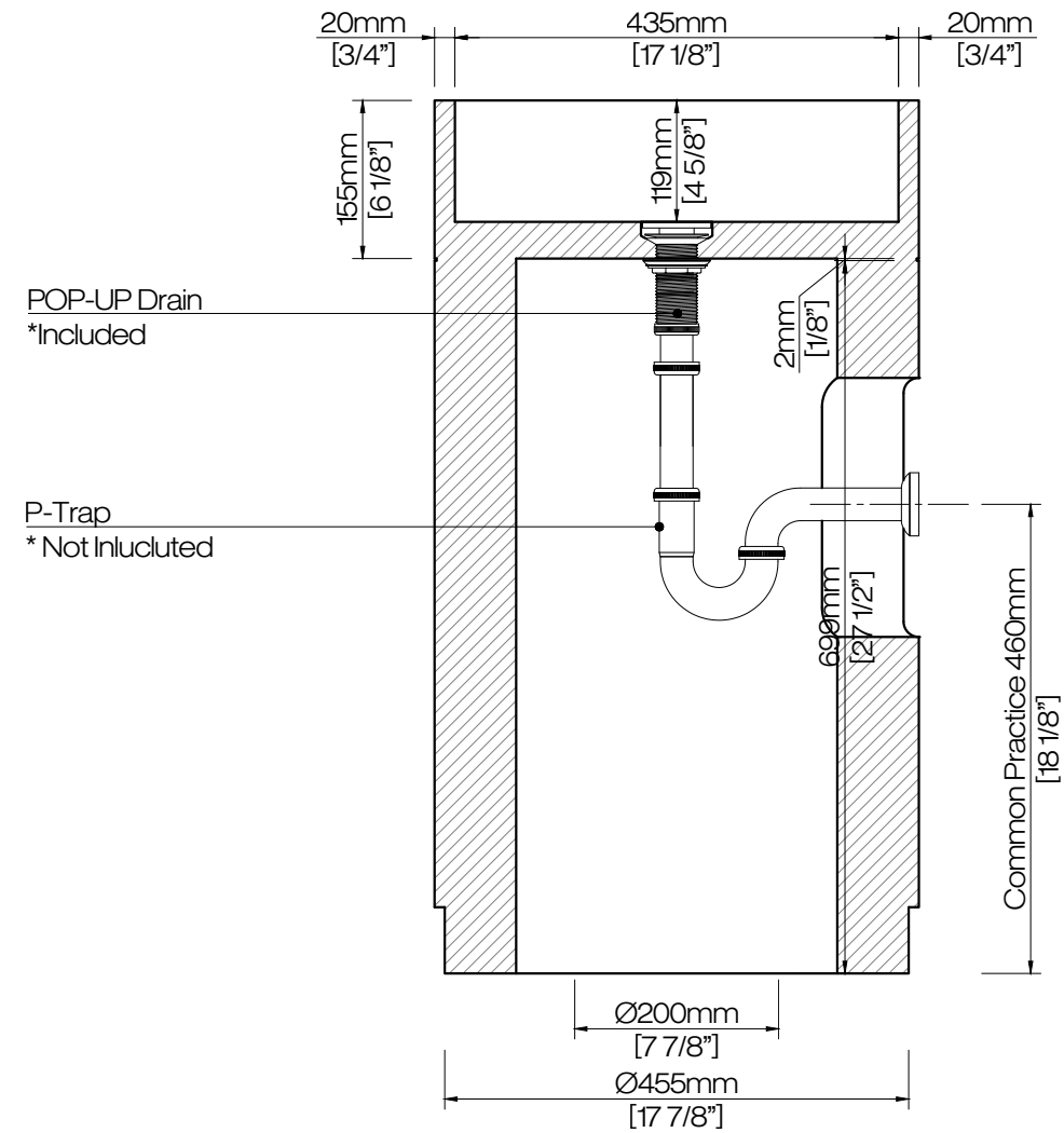
Section b-b
