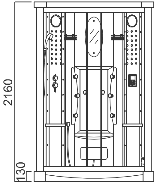
SIZE:1060X1060X2160mm
