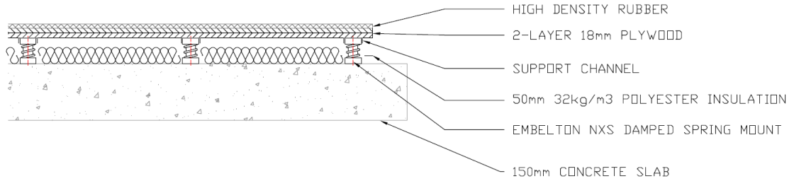
Figure 5: Damped springs with 2-layer 18mm plywood and top surface rubber build-up
