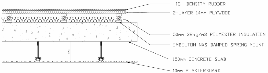
Figure 4: Damped springs with 2-layer 14mm plywood and top surface rubber build-up
