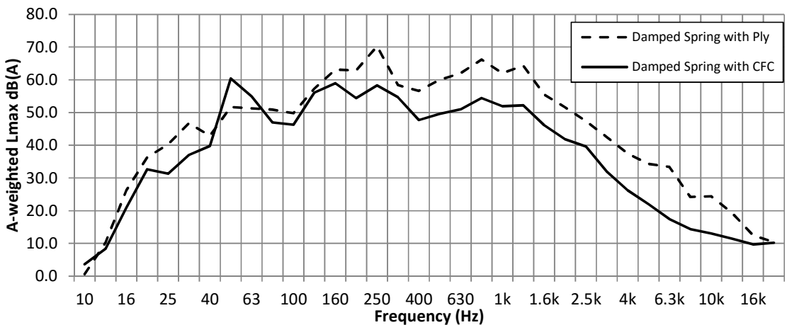
Figure 10: 1/3 Octave L_{max} for Test B floor systems
