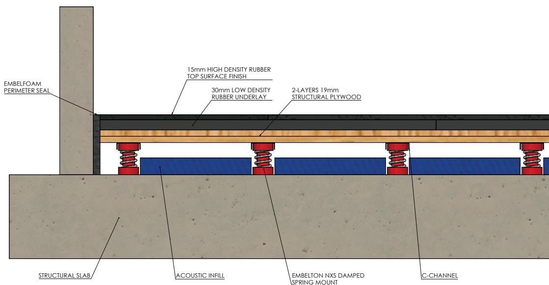
NXS INSTALLATION EXAMPLE
