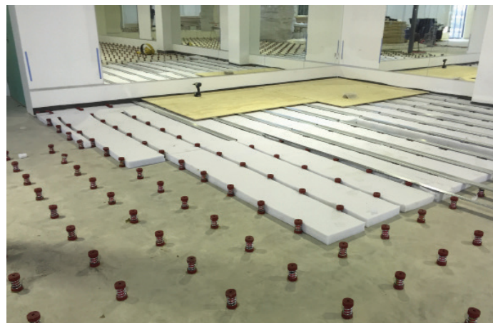
NXS-14 TYPICAL INSTALLATION
