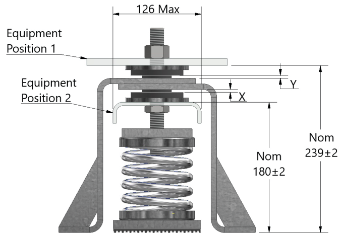
CDM INSTALLATION
