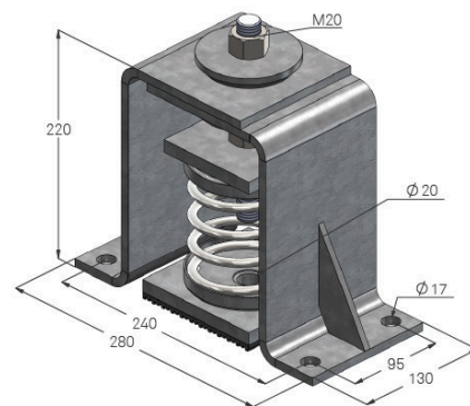
CDM DIMENSIONS
