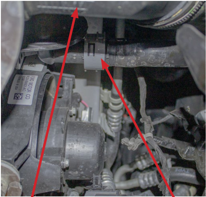
Recirculation tube
