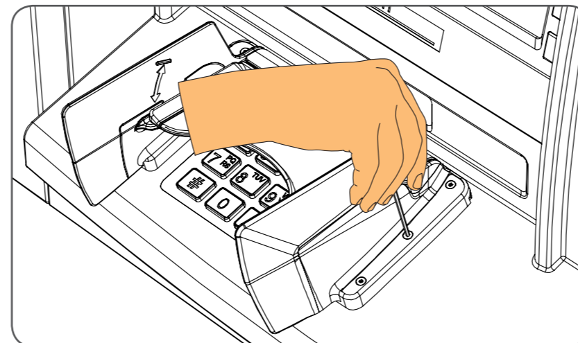
Step 9: Screw the wings down by using the screws provided. Do not over-tighten
