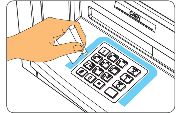
Step 4: Brush the primer onto the area shown. Ensure complete coverage of PINGuard® footprint area. Allow to dry for 5 minutes.
