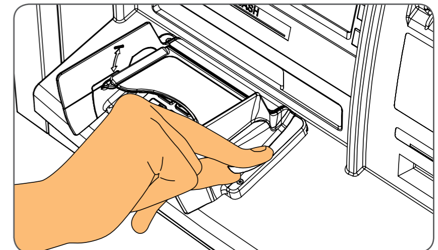
Step 10: Using the cleaning sachet, thoroughly wipe the area around the PINGuard® to ensure that any residue primer is removed. Then finally fit cover labels as shown.
