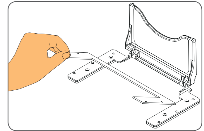
Step 7a: When fitting an EVO1i Recess you will now need to unscrew and remove the U shaped metal bracket.
