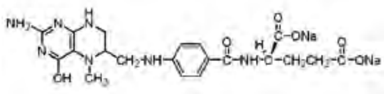
Figure 10. Molecular structure of folate
