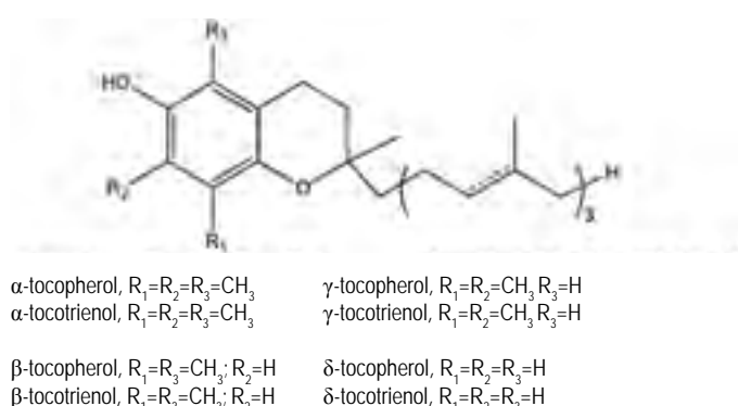
Figure 9. Molecular structures of various forms of Vitamin E
