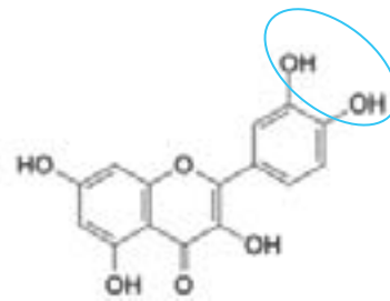
Quercetin
