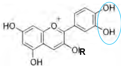
Anthocyanin
