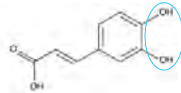
Caffeic acid
