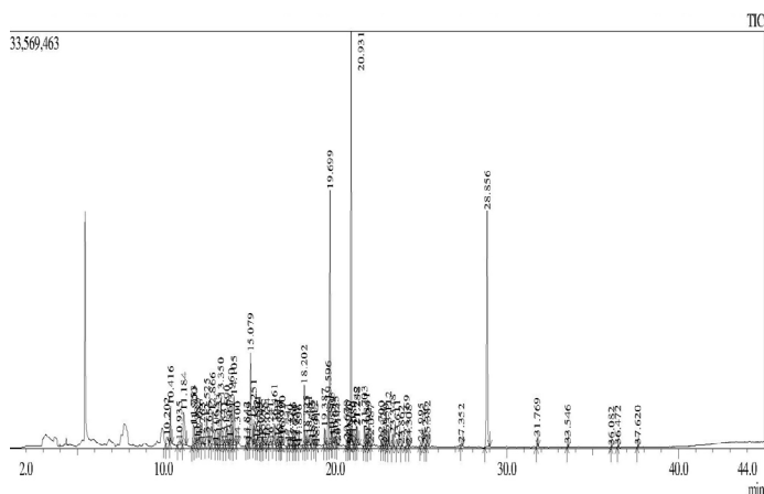
Figure 3: Head space gas chromatogram of 0.5 µL injections of T. ferdinandiana ethyl acetate fruit extract. The extract were dried and resuspended in methanol for analysis.
