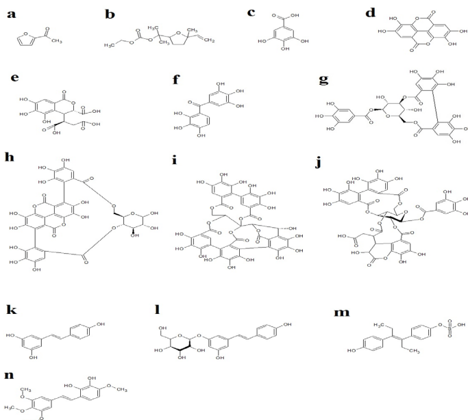
Figure 5: Chemical structures of (a) 1-(2-furanyl)-ethanone, (b) ethyl 2-(5-methyl-5-vinyltetrahydrofuran-2-yl) carbonate, (c) gallic acid, (d) ellagic acid; (e) chebulic acid, (f) galloyl pyrogallol, (g) corilagen, (h) punicalin, (i) castalagin, (j) chebulagic acid, (k) resveratrol, (l) piceid, (m) diethylstilbestrol monosulfate, (n) combretastatin A1.
