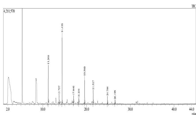
Figure 4: Head space gas chromatogram of 0.5 µL injections of methanolic T. ferdinandiana leaf extract. The extract were dried and resuspended in methanol for analysis.
