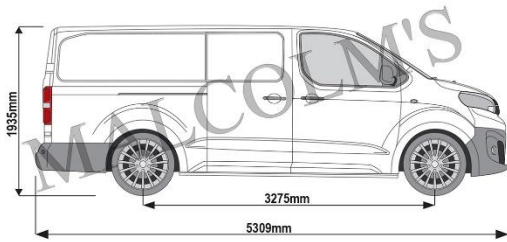
Citroen Dispatch 2016 on L3H1.jpeg
