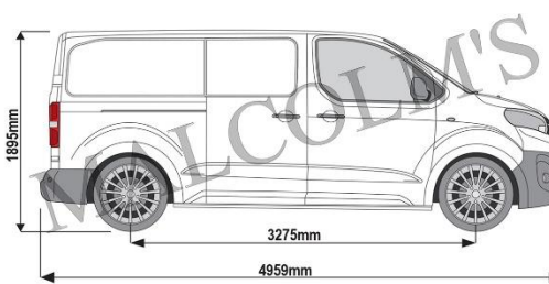
Toyota ProAce 2016 on L2H1.jpeg
