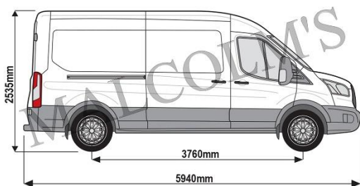
LDV Maxus Deliver 9 2020 on L3H2.jpeg
