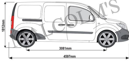
Renault Kangoo 2009-2021 L3H1.jpeg
