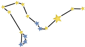
The Dragon
