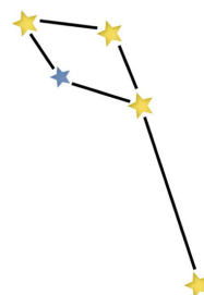
The Dolphin
