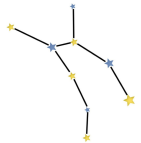
Lupus
