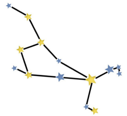
The Herdsman
