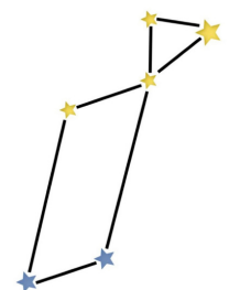
The Harp
