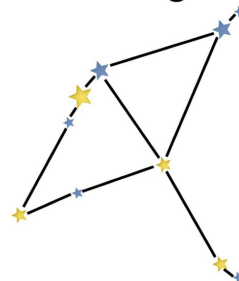
The Eagle
