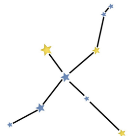
The Swan
