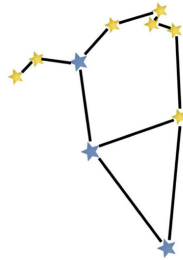
The King
