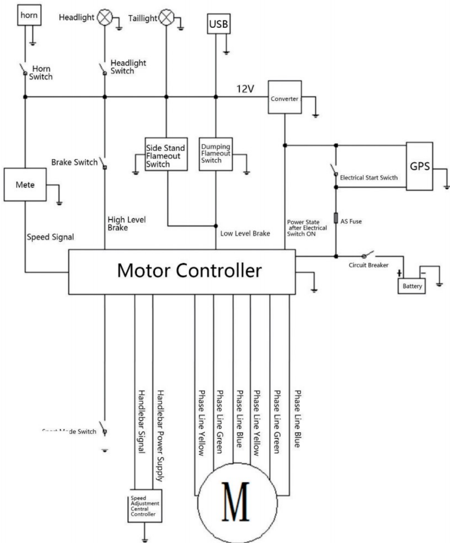
Three Phase Brushless DC Motor
