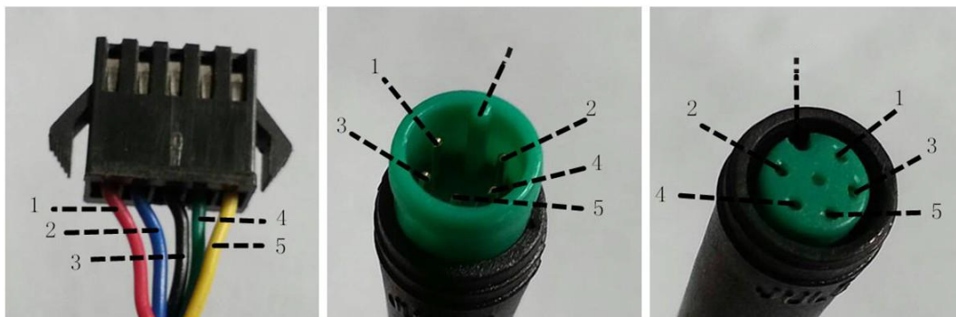
Controller connector
