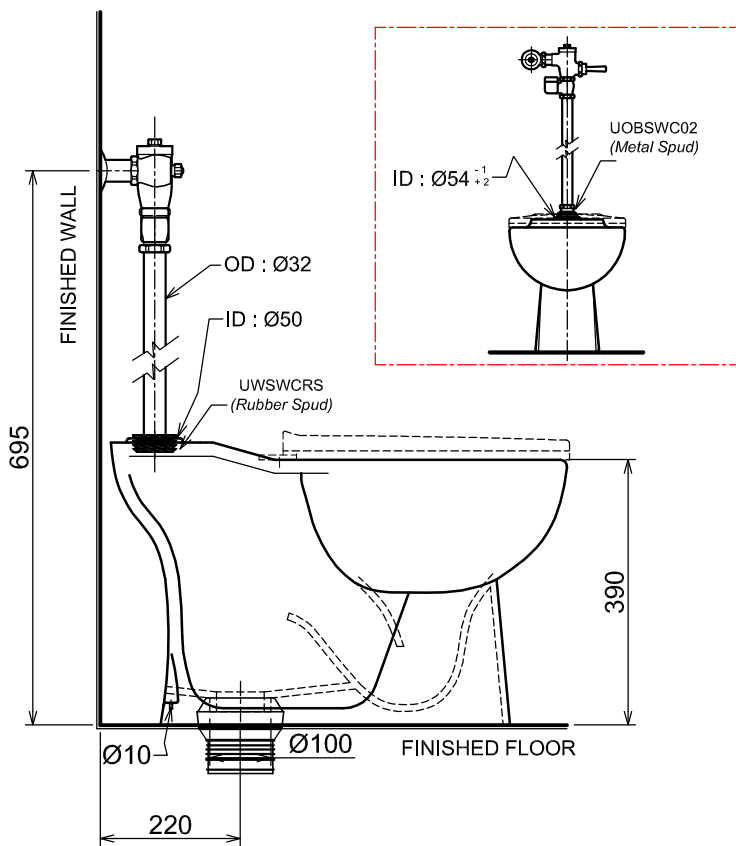
SIDE ELEVATION
