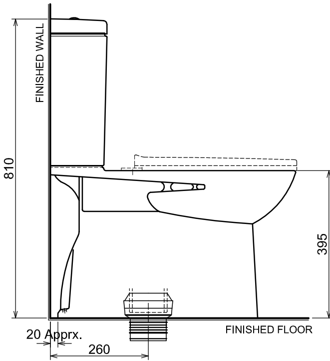
SIDE ELEVATION
